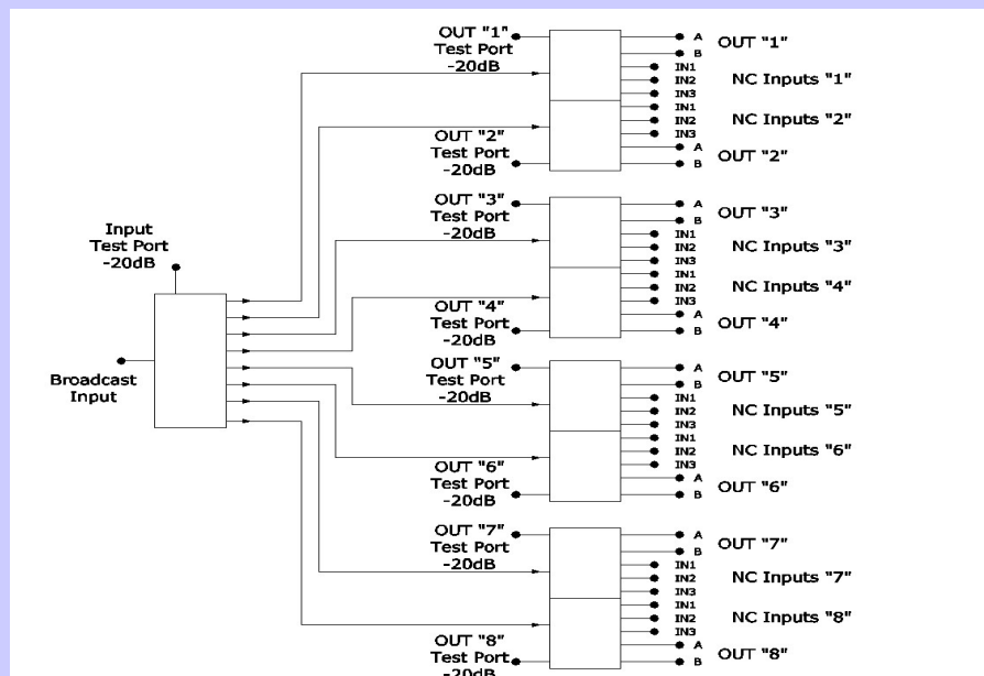
PNF-112 Block Diagram
